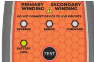
Figure 1.7 Amber LED 1 second flash
