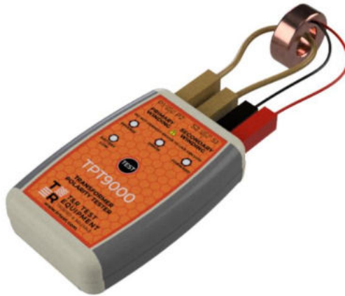
Figure 2.1 TPT9000 connections to a test CT
