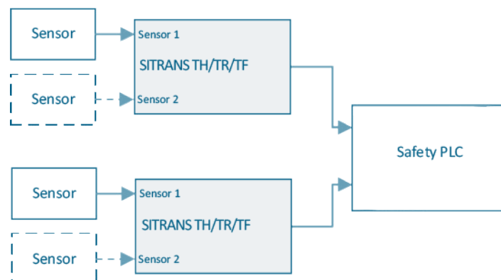
Figure 4 Two transmitter 1oo2 operation (SIL 3)
