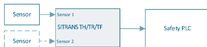
Figure 3 Single transmitter 1oo1 operation (SIL 2)
