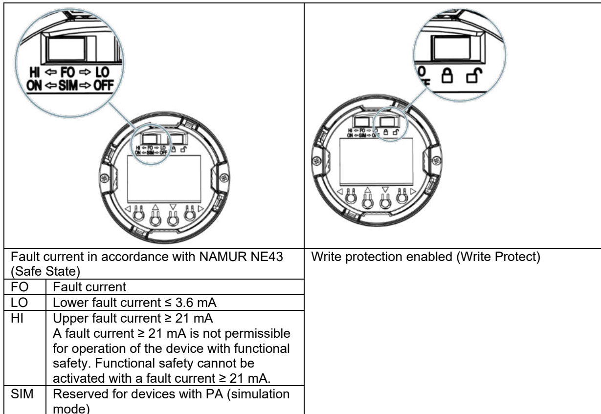
Figure 2 Meaning of the switch positions SITRANS TF and SITRANS TS500 with display
